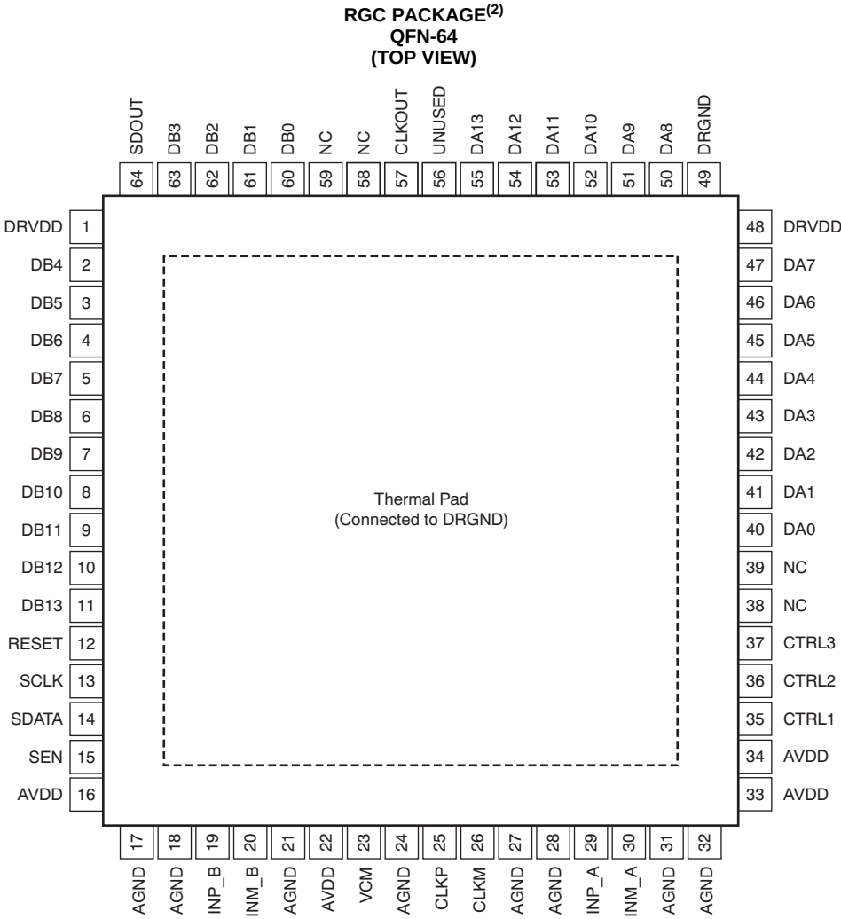
Figure 6. CMOS Mode
