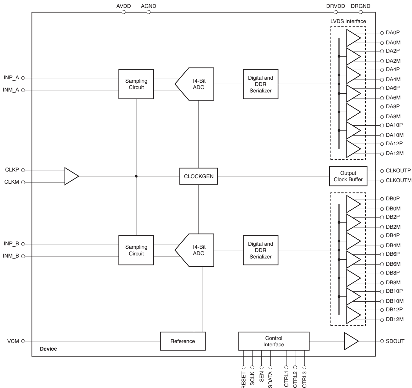
Figure 7. Block Diagram
